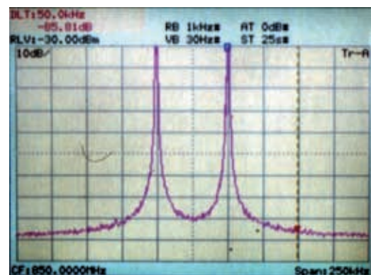
Two-signal third order intermodulation measurement
